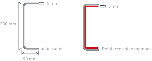
Medium Chassis
